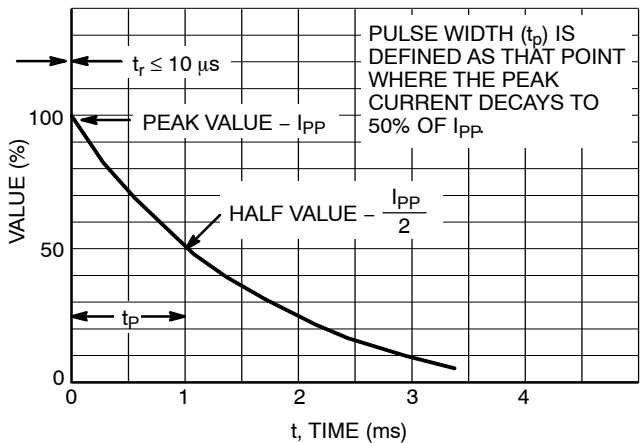
Figure 4. Pulse Waveform
